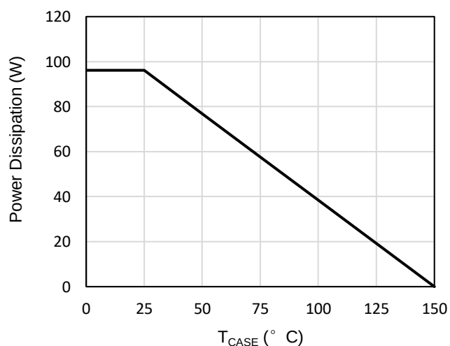
Figure 11: Power De-rating
